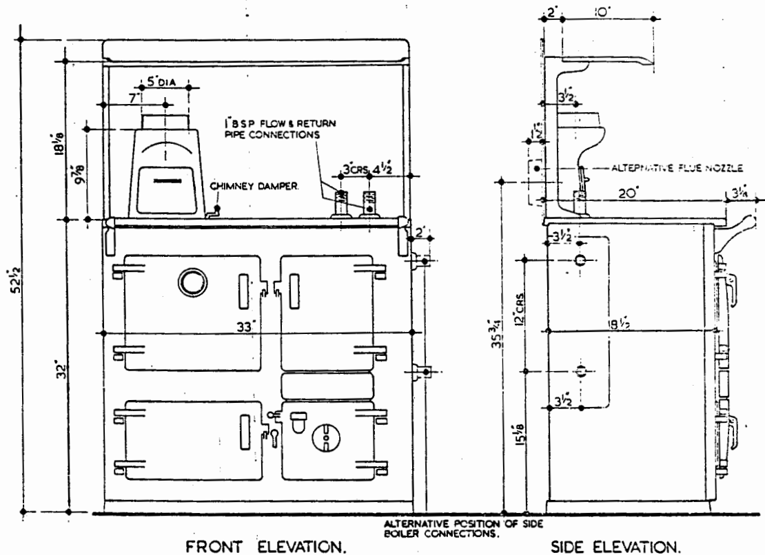
FRONT ELEVATION.
